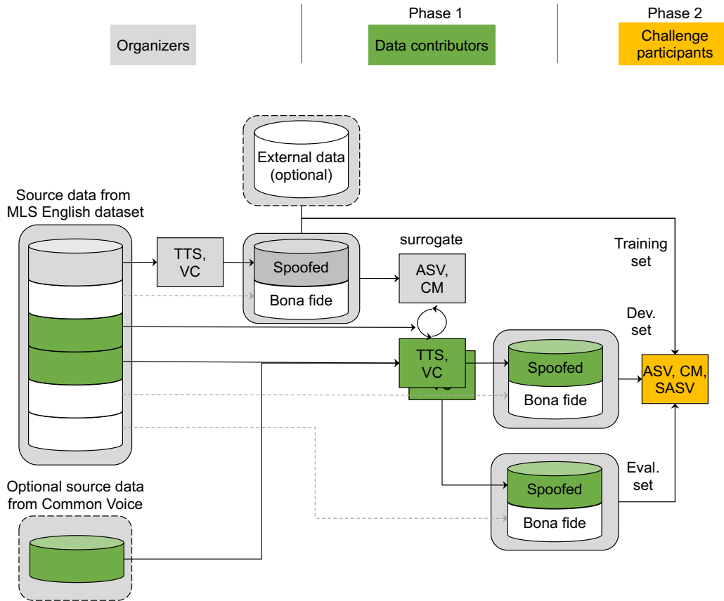
Figure 1: An overview of ASVspoof 5 phases reflecting the roles of organisers (gray-coloured components), data contributors (green) and challenge participants (yellow).
